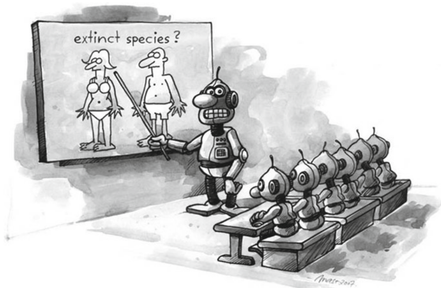
Fig. 8.1 Supervised learning ...
